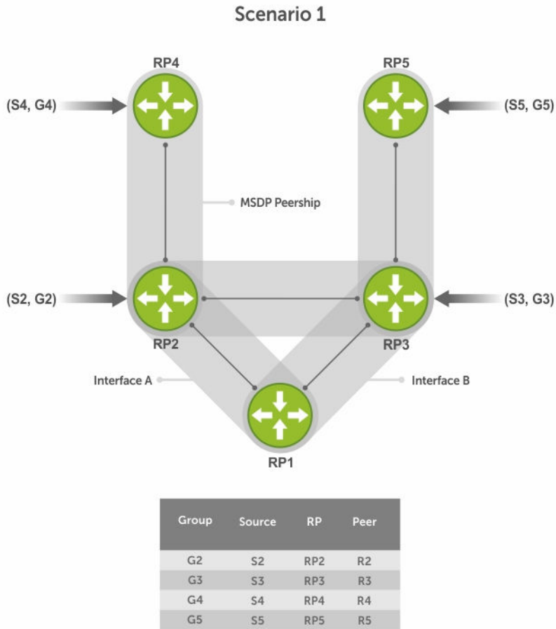
Figure 80. MSDP Default Peer, Scenario 1
